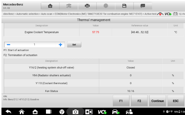
Figure 4-13 Active Test Screen
