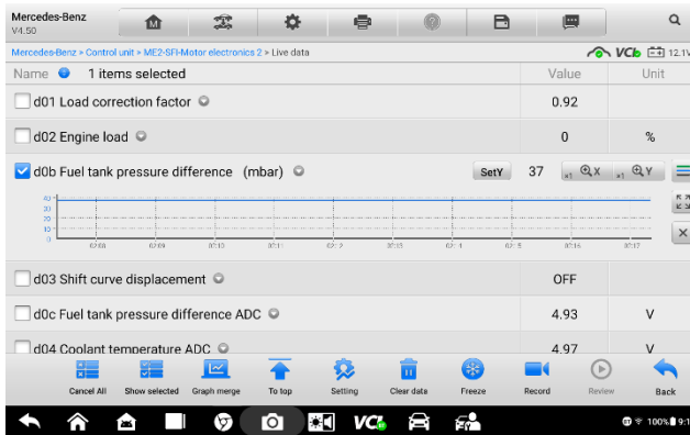
Figure 4-12 Waveform Graph Mode
