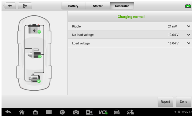
Figure 6-12 Generator Test Result Screen
