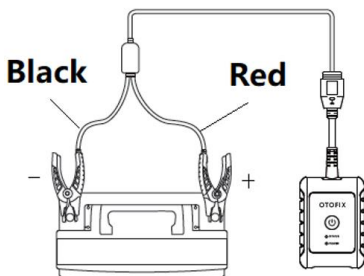
Figure 6-2 Connecting to a Battery
