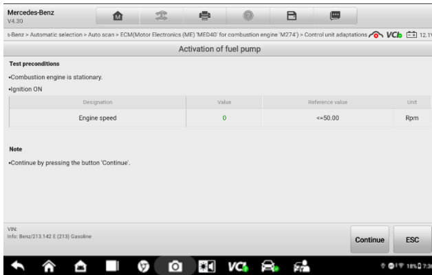
Figure 4-14 Adaptation Operation Screen
