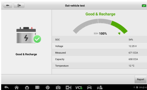
Figure 6-14 Out-vehicle Test Result Screen
