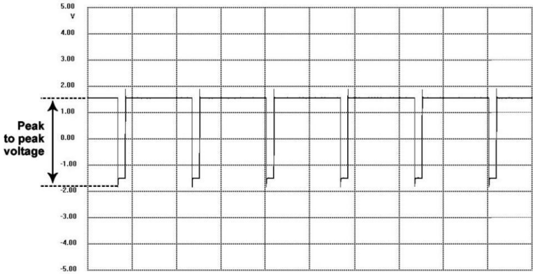
Figure 19-2 Square Waveform
