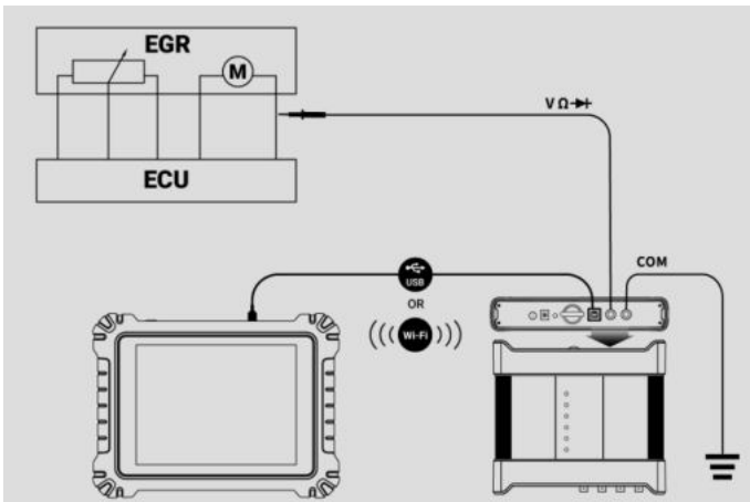
Figure 7-12 Sample Actuator Drive Connection Diagram
