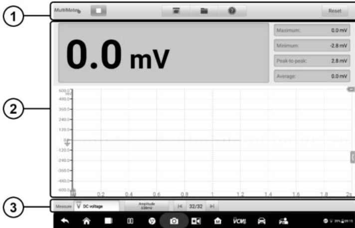
Figure 7-4 Sample Multimeter Menu Screen
