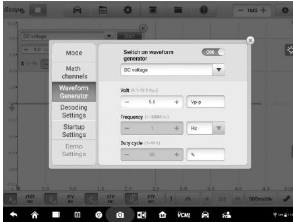
Figure 7-22 Sample Waveform generator Settings Screen
