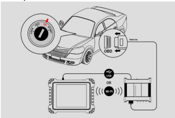
Figure 7-60 Sample DLC Connection Diagram
