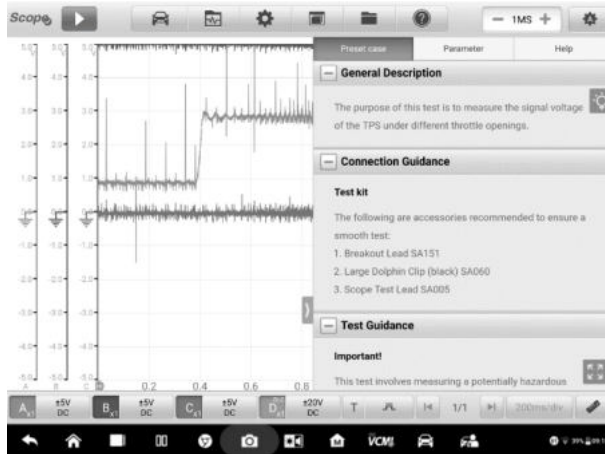
Figure 5-32 Sample Component Measurement Screen 13
