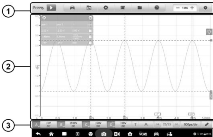
Figure 7-6 Sample Oscilloscope Menu Screen
