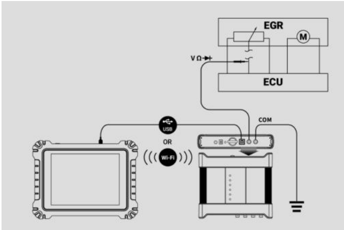
Figure 7-11 Sample DC Voltage Connection Diagram
